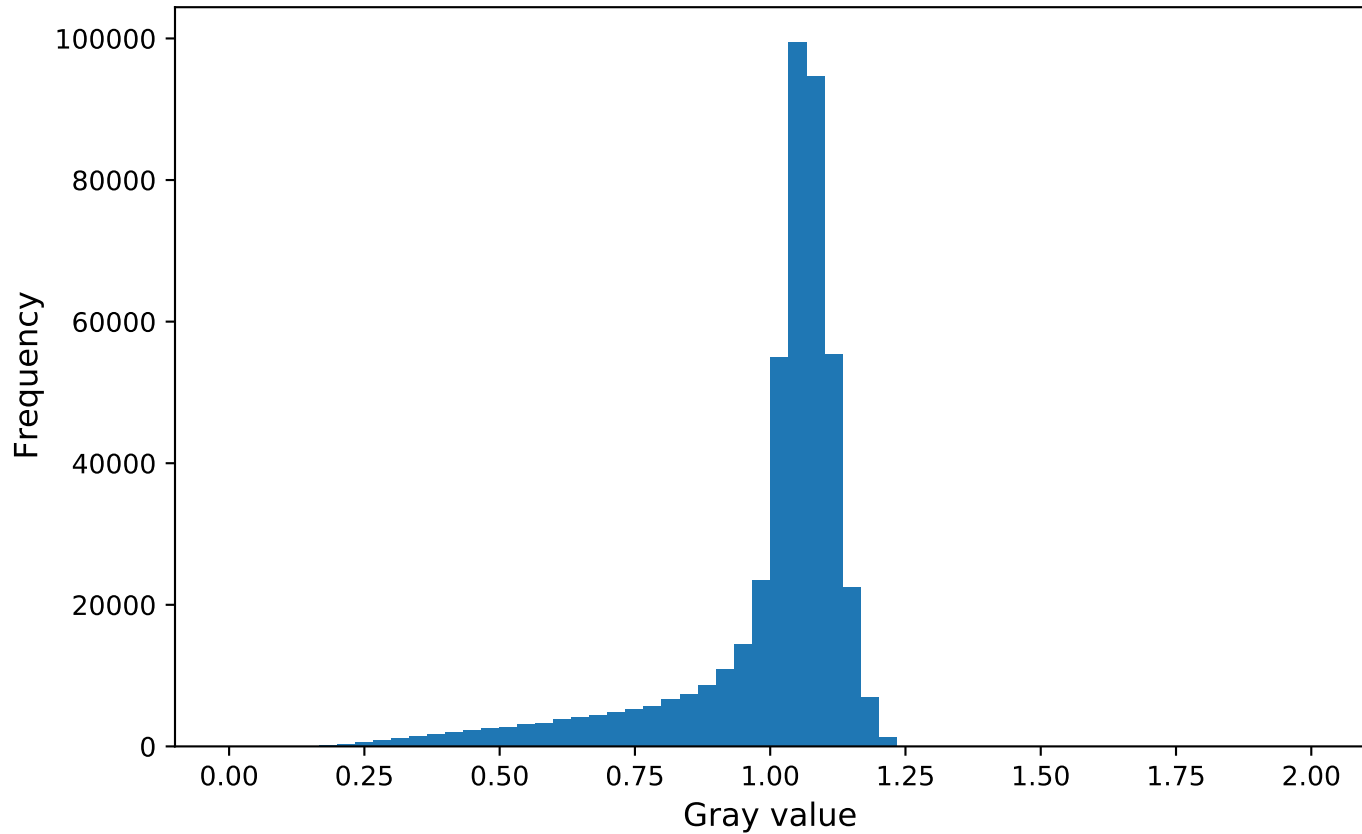
Image Histogram
